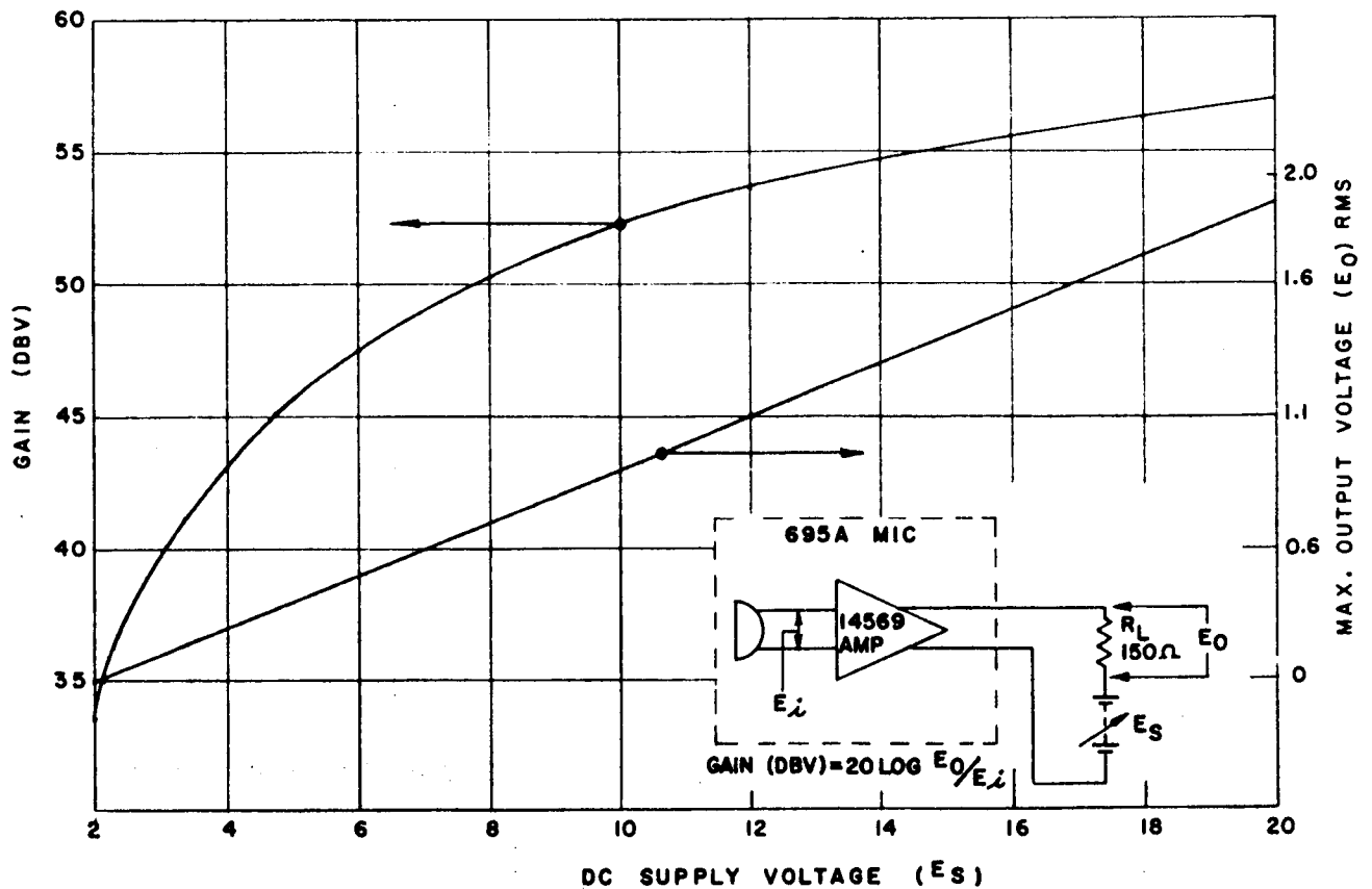
695A MICROPHONE AMPLIFIER (14569 ASSEM.) GAIN AND OUTPUT VS SUPPLY VOLTAGE
