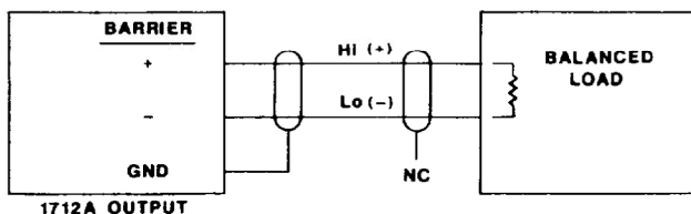
Figure 3. Typical Output Connections
