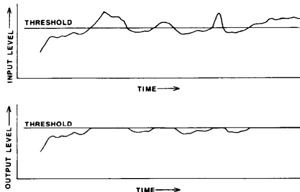
Figure 5. An Input Level and Its Corresponding Output Level at ∞:1 Compression Ratio
