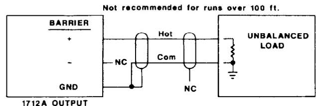
Figure 3. Typical Output Connections
