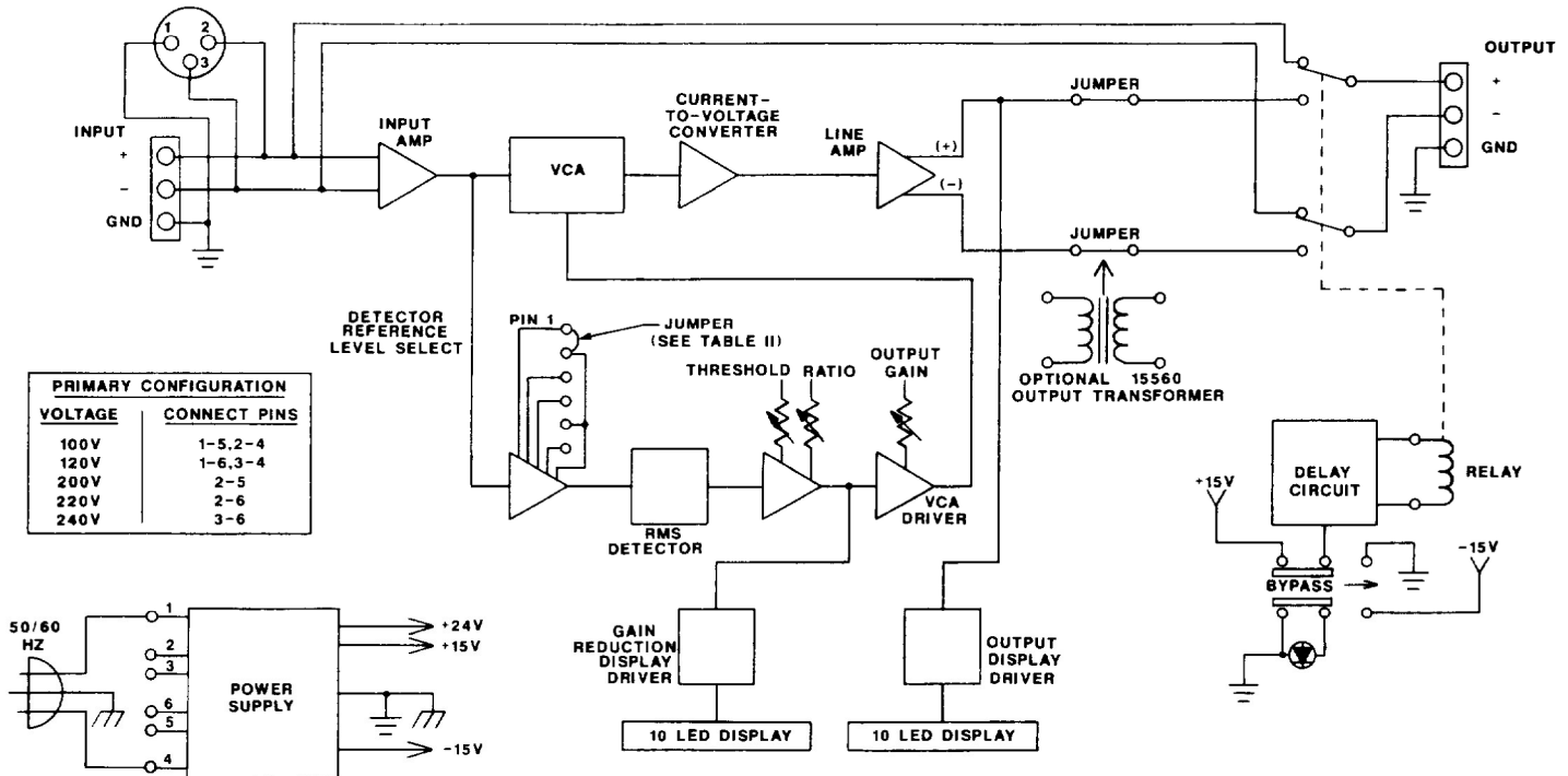
Figure 6. Block Diagram of the 1712A
