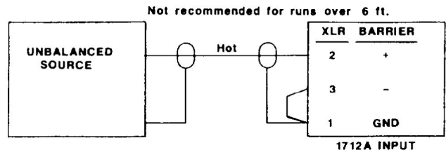
Figure 2. Typical Input Connections
